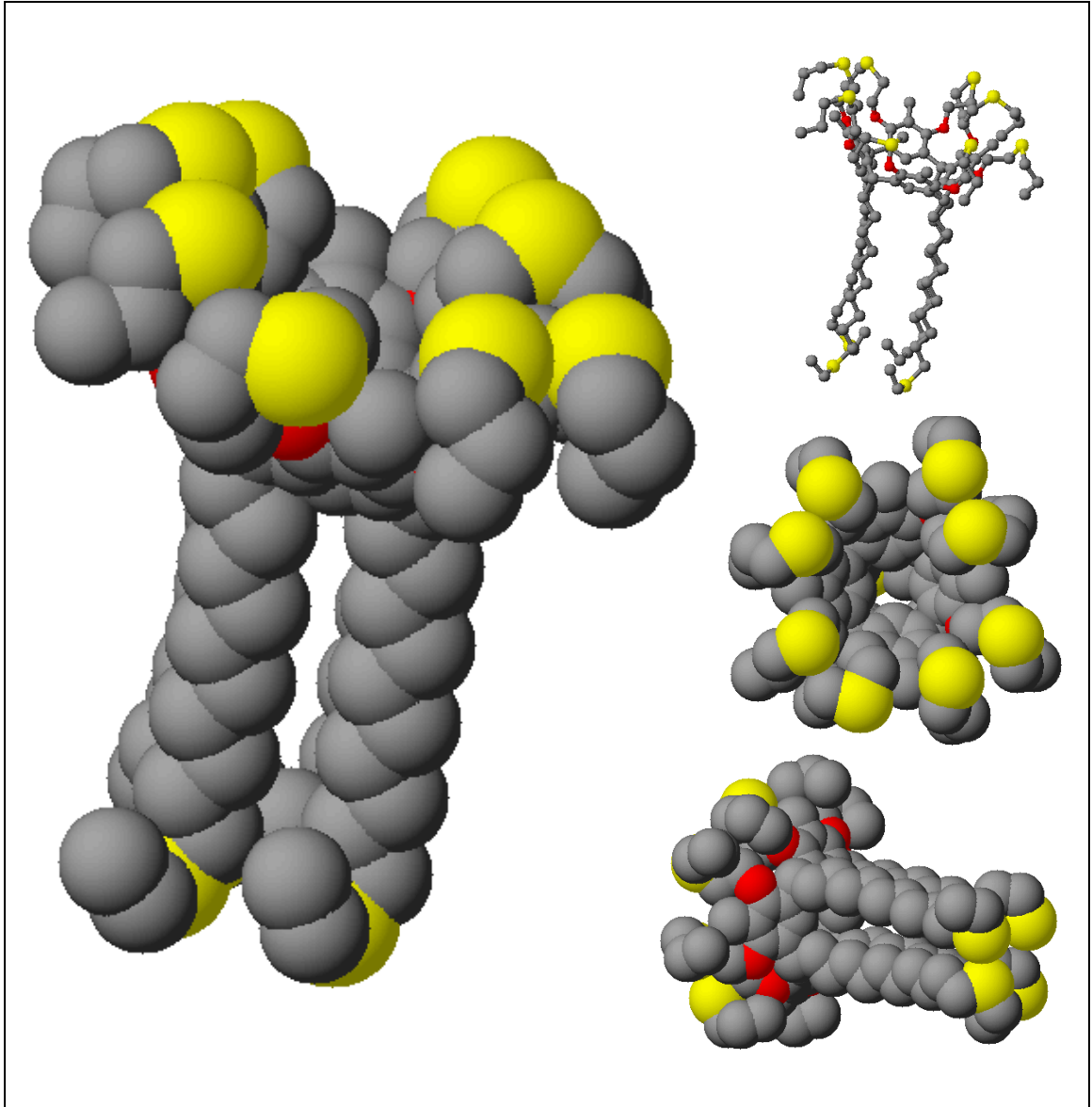
Figure 5.2: 3-D Schematic of Sulfide Modified Resorcinarene Molecule
